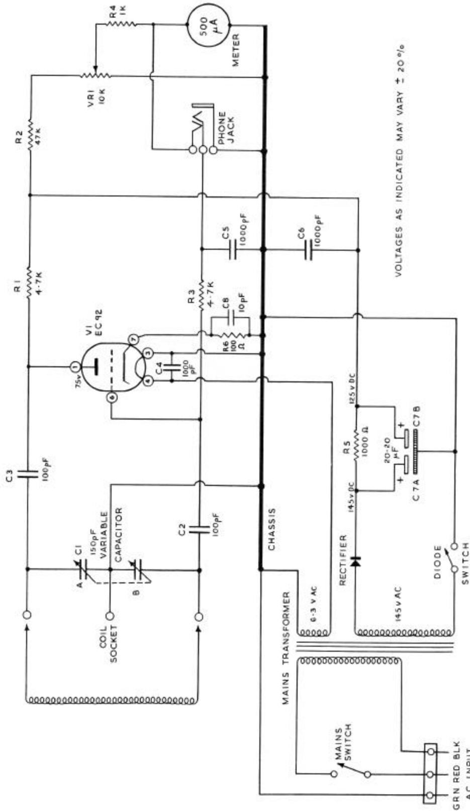
HEATHKIT GRID DIP METER MODEL GD-1U CIRCUIT DIAGRAM
