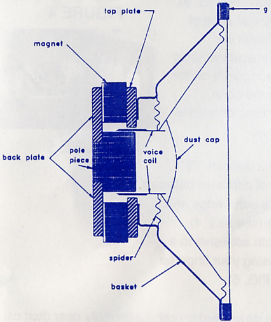
(CROSS SECTION OF LOUDSPEAKER)
